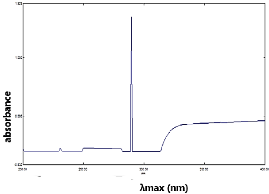
Figure (1): The maximum wavelength of measuring MRT absorbance ( \lambda_{max} ) was 289 nm in phosphate buffer PH 6.8.
