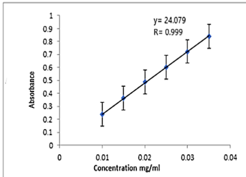
Figure (2): Standard calibration curve of MRT in (PBS) PH 6.8.
