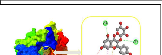
Figure 1. Ligand 6 Docking interactions between protein Human CYP3A4 bound to metformin (PDB ID 5G5J), showing key binding sites and molecular interactions.
